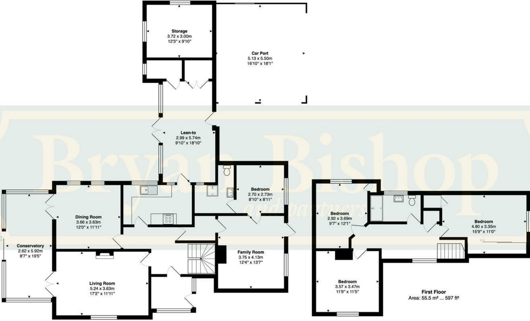
Ground Floor Area: 140.5 m² ... 1513 ft²
